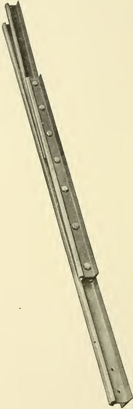
Fig. 236. Typical Steel Track Form. "Mate"
